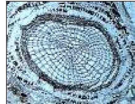
Earliest Fossil
